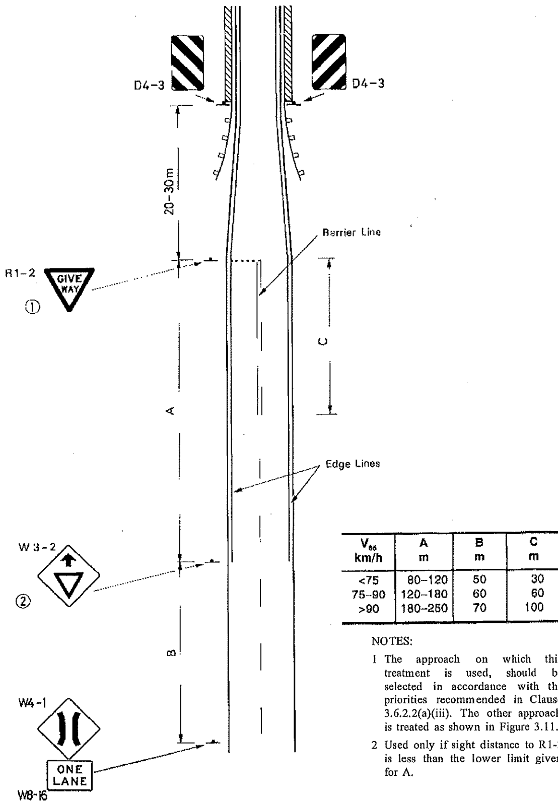
FIGURE 3.12 ONE-LANE BRIDGE WITH GIVE WAY SIGN
