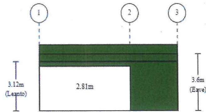
Left Side - South
